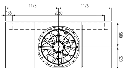
Mod. MC 172-P÷192-P MC/SL 172-P÷192-P
