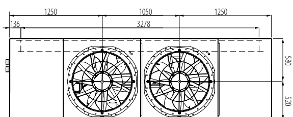
Mod. MC 212-P÷272-P MC/SL 212-P÷272-P MC/SSL 172-P÷212-P
